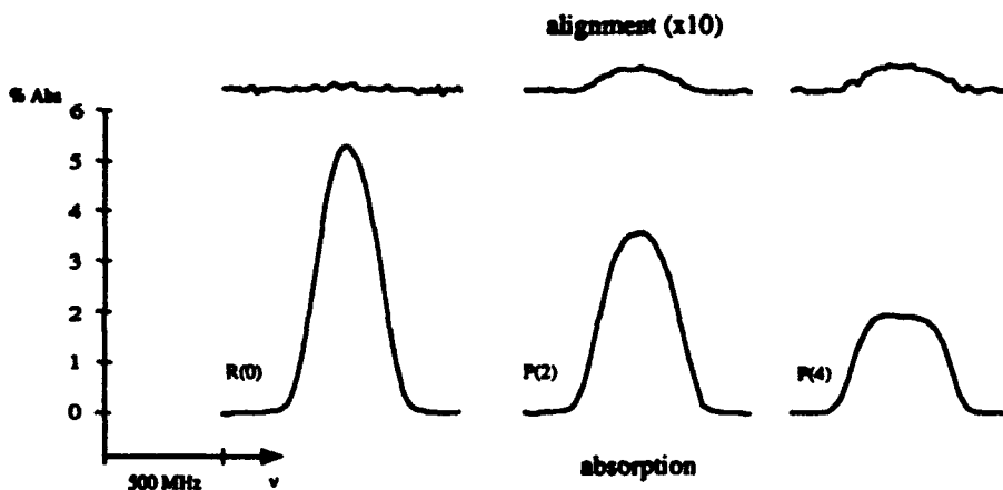
Fig. 6. Typical alignment scans over \text{CO}_2 transitions ( \nu_3 , asymmetric stretch)
